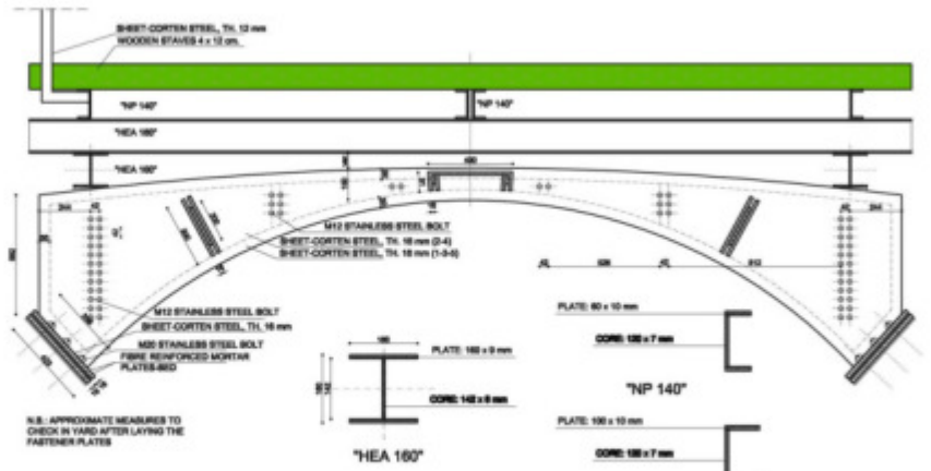
ASSEMBLED SHEET-CORTEN STEEL DETAILS -1 : 5 SCALE-
